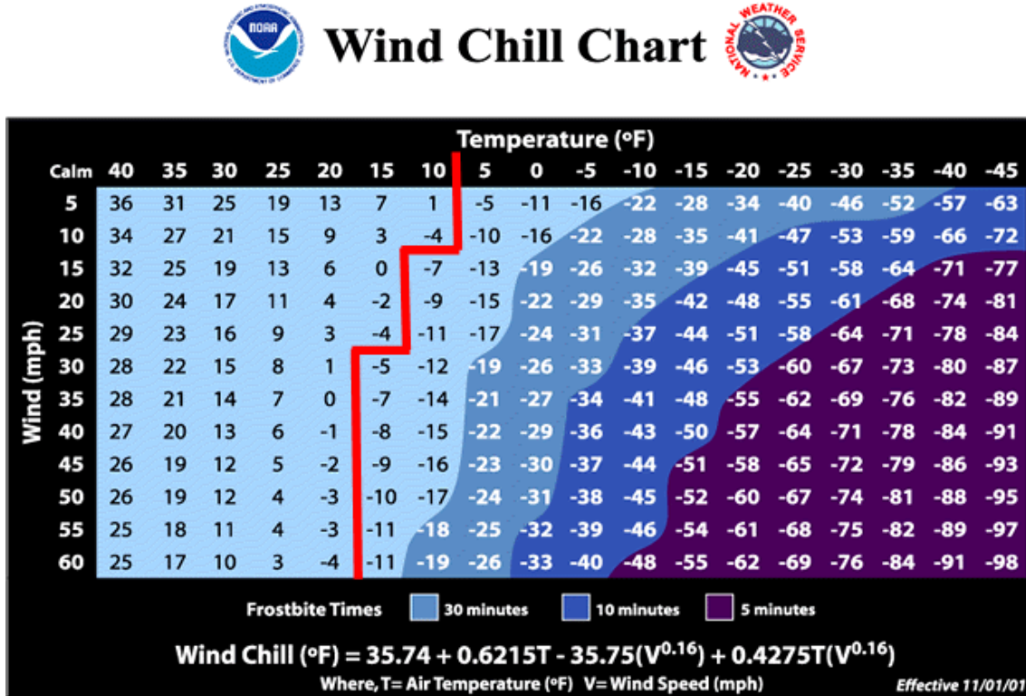
Figure 3 Wind chill chart
